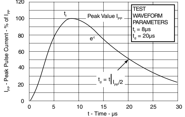
FIGURE 2 PULSE WAVEFORM
